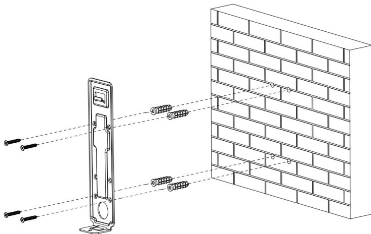
Figure 2-2 (Standard Mount)
